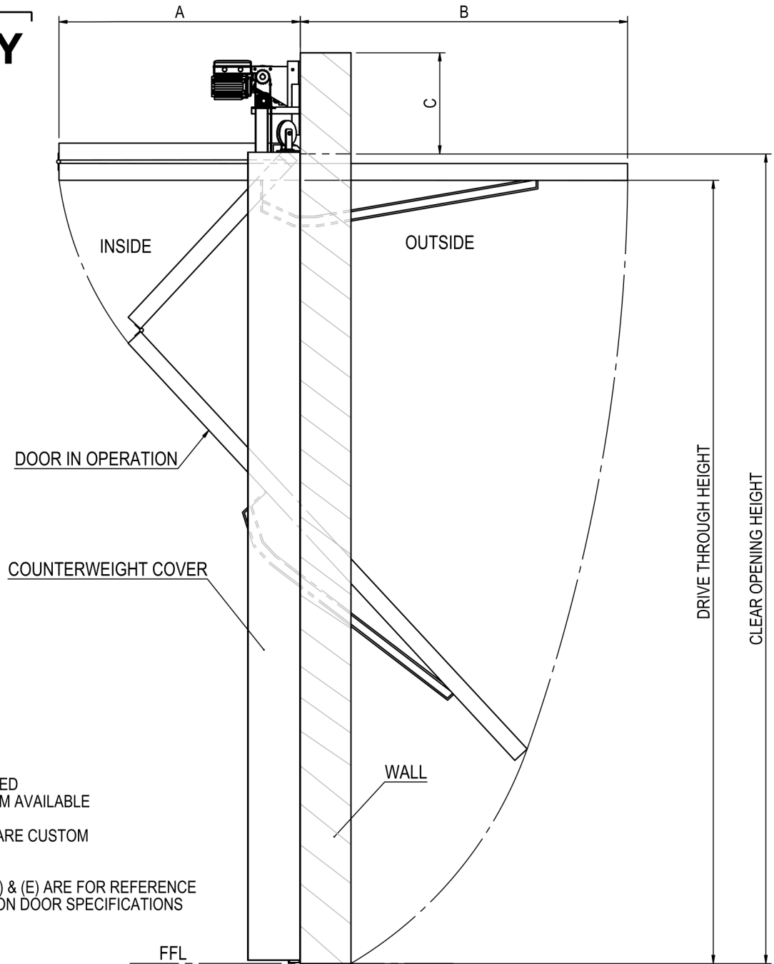
SIDE VIEW
